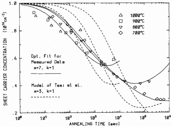
Fig. 23. Measured data of the sheet carrier concentration of [6] at four temperatures. Results due to the cluster model of [5] and an optimal fit to measured data.
