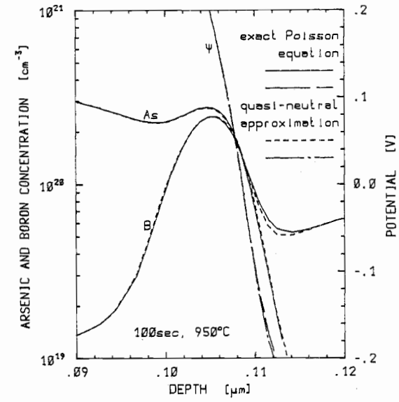
Fig. 5. Arsenic and boron distributions after 100-s inert diffusion at 950°C due to the models P and Q .
