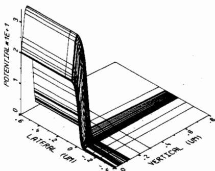
Fig. 12. Two-dimensional distribution of the electrostatic potential after an inert diffusion of 10 s at 1000°C.
