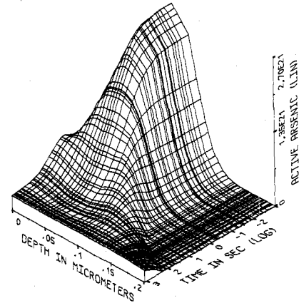
Fig. 19. Transient dependence of the electrically active arsenic during a 20 min annealing step at 1000°C.
