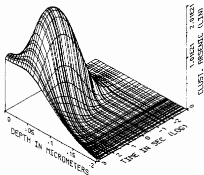
Fig. 20. Transient dependence of the clustered arsenic concentration during a 20-min annealing step at 1000°C.
