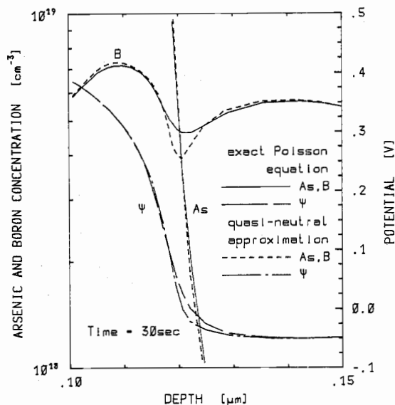
Fig. 11. Arsenic, boron, and the electrostatic potential due to the models P and Q for an inert diffusion at 1000°C after 30 s.
