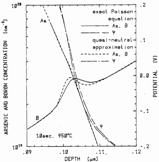
Fig. 3. Arsenic and boron distributions after 10-s inert diffusion at 950°C due to the models P and Q .
