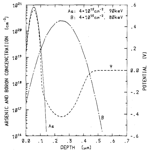
Fig. 1. Arsenic and boron profile after ion implantations. As: 4 \times 10^{15} \text{ cm}^{-2} with 90 keV, LSS, Gaussian; B: 4 \times 10^{15} \text{ cm}^{-2} with 80 keV, LSS, Gaussian. The electrostatic potential is computed from the exact Poisson equation at 950^\circ\text{C} .
