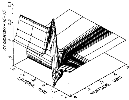
Fig. 17. Two-dimensional distribution of the boron concentration after an inert diffusion of 1500 s at 1000°C.
