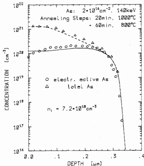
Fig. 21. Total and electrically active arsenic concentrations after two annealing steps.
