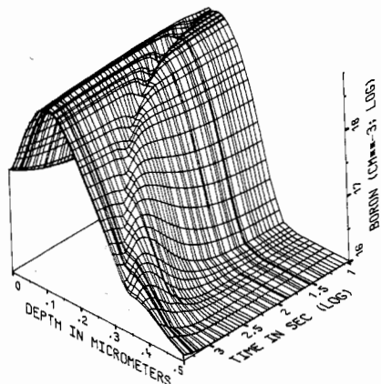
Fig. 8. Time-dependent boron profile for an inert diffusion step of 40 min at 1000°C. The initial distribution has been obtained by ion implantations. As: 4 \times 10^{15} \text{ cm}^{-2} , 90 keV and B: 7 \times 10^{13} \text{ cm}^{-2} , 40 keV.
