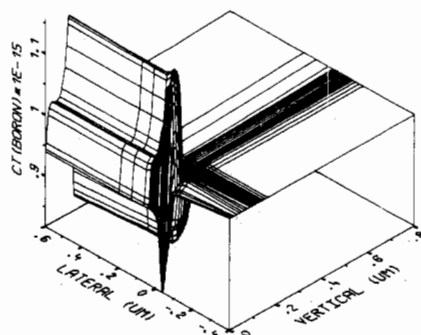
Fig. 14. Two-dimensional boron distribution after an inert diffusion of 100 s at 1000°C.
