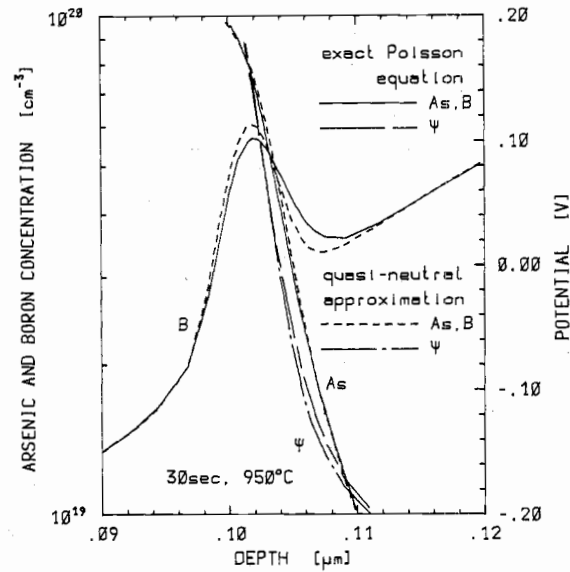
Fig. 4. Arsenic and boron distributions after 30-s inert diffusion at 950°C due to the models P and Q .
