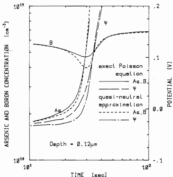
Fig. 10. Time dependence of arsenic, boron and the electrostatic potential due to the models P and Q for an inert diffusion at 1000°C at a depth of 0.12 μm.
