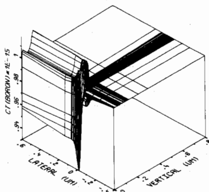
Fig. 13. Two-dimensional distribution of the boron dopants after an inert diffusion of 10 s of 1000°C.
