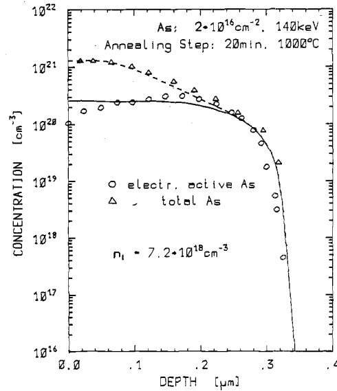
Fig. 18. Measured and computed data of the total and electrically active arsenic concentration after a 20-min annealing step at 1000°C.
