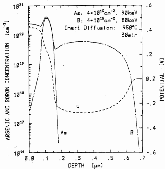
Fig. 2. Arsenic and boron distribution and electrostatic potential after an inert diffusion step of 30 min at 950°C. The initial distribution is given in Fig. 1.
