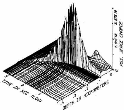
Fig. 9. Transient behavior of the positive space charge density which is defined as the maximum of 0 and n - p + N_A - N_D for the process of Fig. 8.
