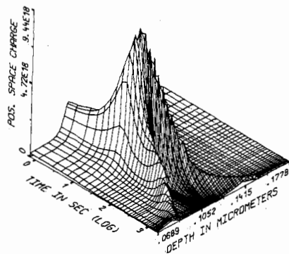
Fig. 6. Time dependent survey of the positive space charge density which is defined as the maximum of \psi and n-p+N_A-N_D in the vicinity of the p-n junction for an inert diffusion step at 950°C. Initial and final distribution are given by Figs. 1 and 2, respectively.
