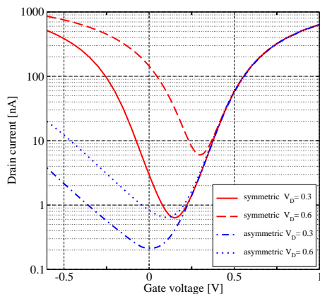
Figure 3: Drain current versus gate voltage from 2D simulations.
