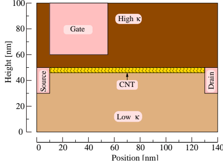
Figure 1: 2D sketch of the asymmetric structure.
