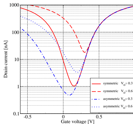
Figure 4: Drain current versus gate voltage from 3D simulations.
