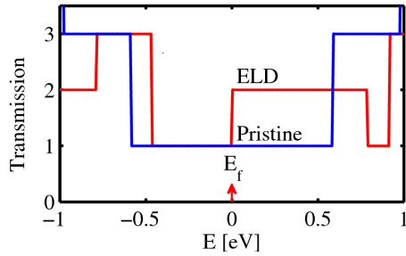
Fig. 2. The transmission function for ZGNR(20) and ELD-ZGNR(10,10)
