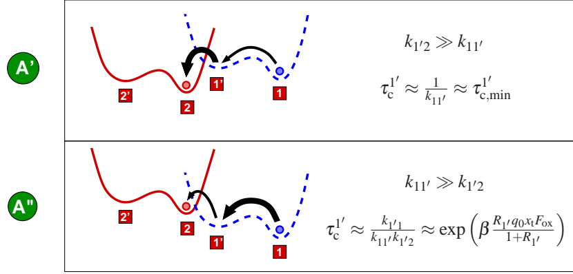
Fig. 17 (PRINT IN COLOR) The same as in Fig. 16 but for the regimes A' and A'' of the oxide field dependence of \tau_c^{1'} .
