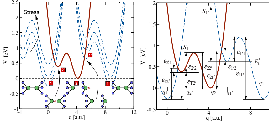
Fig. 13 (PRINT IN COLOR) Left: A schematic of the configuration coordinate diagram for a bistable defect. The solid and the dashed lines represent the adiabatic potentials for a defect in its positive and neutral charge state, respectively. The energy minima correspond to the stable or metastable defect configurations, labeled 1, 1', 2, and 2'. The present configuration coordinate diagram describes the exchange of holes with the valence band and thus is associated with a hole capture or emission process. The stick-and-ball models display a defect in its various stable and metastable configurations for illustration purpose. Right: Definitions of the used energies and barriers in the multi-state model. Recall that two adiabatic potentials must be shown for one transition. It is assumed that an alternative transition pathway with an additional crossing point exists in the multi-dimensional atomic configuration space. In order to show both intersections (related to the transitions 1 \leftrightarrow 2' and 2 \leftrightarrow 1' ) in one configuration coordinate diagram, the 'neutral' potential must be plotted twice. Obviously, \varepsilon_{22'} = \varepsilon_{22} + \varepsilon_{T2'} holds.
