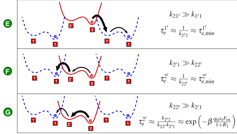
Fig. 18 (PRINT IN COLOR) The same as in Fig. 16 but for the regimes E, F, and G of the oxide field dependence of \tau_e .
