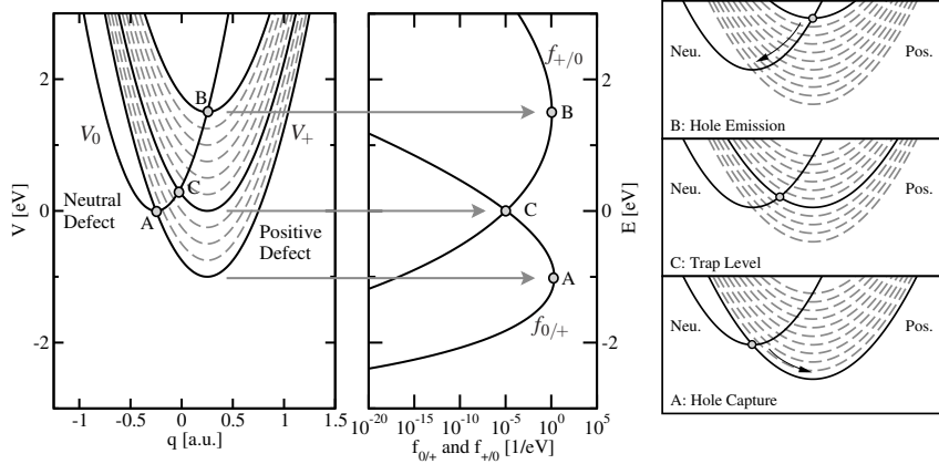
Fig. 6 Configuration coordinate diagram (left) for a continuum of adiabatic potentials V_{\pm}(q) , the corresponding lineshape functions (middle), and sketches of the cases A, B, and C (right). For hole capture, the lineshape function f_{0/+}(E) reaches its maximal value when V_+(q) intersects the minimum of V_0(q) and thus the NMP transition has a vanishing barrier V_{0/+} (case A). When changing from the configuration coordinate diagram (left) to the lineshape function (middle), the adiabatic potentials are converted to electron energies according to equation (23). For the hole emission, the analogous considerations apply as for hole capture. Now the intersection point must lie in the minimum of V_+(q) , giving rise to the peak of the lineshape function f_{+/0}(E) (case B). If the minima of both parabolas coincide, the barriers for both directions have the same heights, which leads to equaling NMP transition rates (case C).
