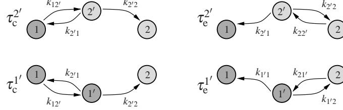
Fig. 12 Simplified state diagrams of hole capture and emission over the metastable states 1' and 2' . The superscripts of \tau denote the intermediate state, which has been passed through during a complete capture or emission event. Note that there exist two competing pathways for a hole capture event, namely one over the intermediate state 1' and one over 2' . Of course, the same holds true for a hole emission event.
