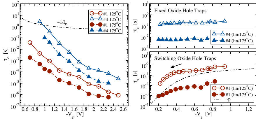
Fig. 1 (PRINT IN COLOR) Left: The capture time constants \tau_c as a function of V_g for two defects at different temperatures extracted from a single device. Open and closed symbols mark measurements carried out at 125°C and 175°C, respectively. The \tau_c curves show a strong field acceleration and temperature activation. However, the observed field acceleration does not follow the 1/I_d \approx 1/p dependence (dot-dashed line) as predicted by the conventional SRH model. Right: The emission time constants \tau_e for single defects gathered from the TDDS for varying recovery gate voltages. The two distinct field dependences (upper and lower panel) suggest the existence of two types of defects present in the oxide. The defect #1 shows different field behaviors depending on whether the device is operated in the linear or the saturation regime during the measurement (not shown here). This suggests that the electrostatics within the device are responsible for the two distinct field dependences. It is noteworthy that the drop in \tau_e goes hand in hand with the decrease in the interfacial hole concentration p (dot-dashed line).
