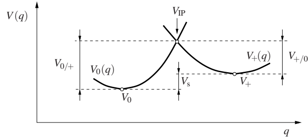
Fig. 9 The hole capture ( V_{0/+} ) and emission ( V_{+/0} ) barrier for an NMP transition. The barrier heights are calculated as the energy differences between the corresponding minimum and the intersection point in the hole picture, which yields V_{0/+} = V_{IP} - V_0 = V_{IP} - \tilde{V}_0 + E and \Delta V_{+/0} = V_{IP} - V_+ = V_{IP} - \tilde{V}_0 + E_t for the capture and the emission barrier, respectively.
