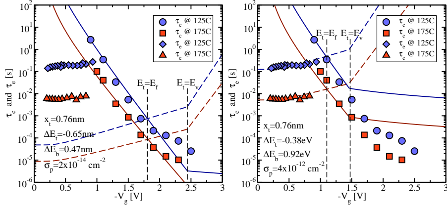
Fig. 2 (PRINT IN COLOR) Two fits of the Kirton model to the TDDS data. The symbols stand for the measurement data and the lines represent the simulated time constants. Left: When the Kirton model is optimized to the hole capture times \tau_c , reasonable fits can be achieved but \tau_e is predicted three orders of magnitudes too low. Right: Alternatively, a good agreement can be obtained for the hole emission times \tau_e but with a strong mismatch of the capture times \tau_c for E_t > E_v . From this it is concluded that the Kirton model is not capable of fitting \tau_c and \tau_e at the same time.
