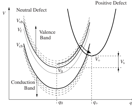
Fig. 7 The same configuration coordinate diagram as in Fig. 5 but in the ‘hole picture’. Note that the energy scale of the charge carriers and thus the band diagram is inverted compared to the ‘electron picture’. Furthermore, the energy of the transferred charge carrier is now undefined for the initial state since the hole is in one of the valence band states. By contrast, it can be specified by E_t when the hole is trapped.
