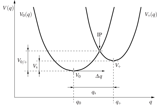
Fig. 4 The configuration coordinate diagram for an NMP transition. The adiabatic potentials for the initial and the final states are denoted V_0(q) and V_+(q) , respectively. They are defined by their corresponding minima V_0 and V_+ located at their equilibrium configurations q_0 and q_+ , respectively. To simplify the mathematical calculations, the axis origin is shifted into the energy minimum V_0 .
