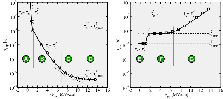
Fig. 15 (PRINT IN COLOR) Left: The calculated hole capture time constants as a function of the oxide field. The different regimes of \tau_c (A, B, C, and D) are separated by the thin vertical lines and labeled by the circles with the capital letters. The dotted curves \tau_c^i show the capture processes over a metastable state i . The field dependence of \tau_c within a certain regime is shown by the dashed curve. Right: The same but for the hole emission time constants with the regimes (E, F, and G).
