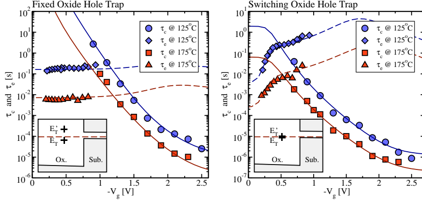
Fig. 14 (PRINT IN COLOR) Left: The capture (solid lines) and emission (dashed lines) times of a fixed oxide hole trap as a function of the gate bias. The symbols stand for the measurement data and the lines represent the simulation results of the multi-state model. The latter are shown to be in remarkable agreement with the experimental data. The inset (bottom left) depicts the band diagram of a MOSFET with the trap levels E_t and E_t' for the case when no bias is applied to the gate. Under these conditions the trap level E_t' is located far above the substrate Fermi level and the emission time remains unaffected by the gate bias. This fact eventually characterizes this defect as a fixed oxide hole trap Right: The same but for a switching oxide hole trap as presented in the Section 2. Compared to the fixed oxide hole trap, it shows a strong gate bias dependence of \tau_c at small gate biases. In contrast to a fixed oxide hole trap, the Fermi level and the trap level E_t' coincide there, resulting in the strong sensitivity of \tau_c to V_g .
