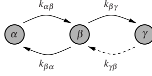
Fig. 11 The state diagram for a two-step process from the state \alpha to \gamma . The first passage time of such a process is calculated by equation (59). Consider that the transition rate k_{\gamma\beta} , indicated by the dashed arrow, does not enter this equation.
