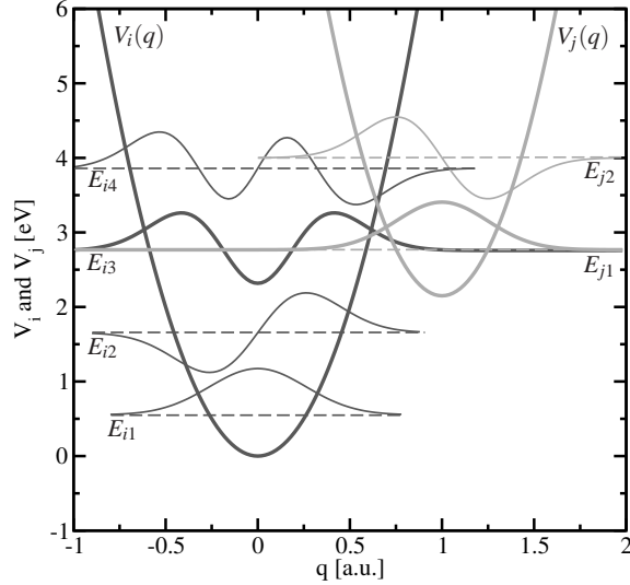
Fig. 3 Adiabatic potentials involved in a charge transfer reaction. Each of the two parabola corresponds to one charge state of the defect where the left ( V_i ) one represents the initial and the right ( V_j ) one the final charge state. Their corresponding wavefunctions and eigenenergies are depicted as solid and dashed lines, respectively. An NMP transition only occurs when the initial and the final energies coincide as it is the case for E_{i3} and E_{j1} . Then the overlap of their corresponding vibrational wavefunctions enters the calculation of the lineshape function f_{ij} and consequently determines the NMP transition probability.
