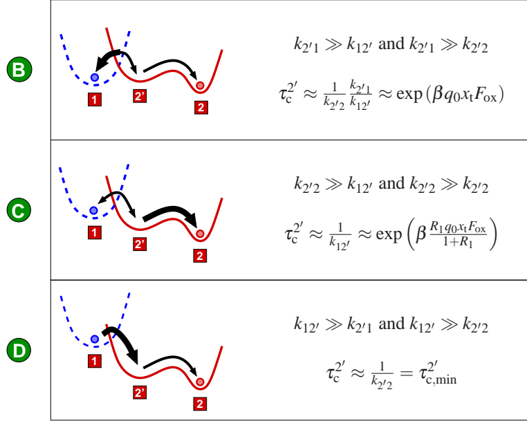
Fig. 16 (PRINT IN COLOR) A schematic representation of adiabatic potentials in the regimes B, C, and D. The arrows show the transitions involved in the hole capture process. Their thicknesses indicate the magnitude of their rates. This means that the thinner arrows are associated with larger transition times and thus governs the oxide field and temperature dependence of the complete capture process T_{1 \rightarrow 2} . With higher oxide fields (B \rightarrow D) the potential of the neutral defect (dashed line) is raised relative to that of the positive defect (solid line). This is associated with an increase of k_{12'} and a decrease of the reverse rate k_{2'1} . In contrast to the charge transfer reactions T_{1 \rightarrow 2'} and T_{2 \rightarrow 1'} , the thermal transition T_{2' \rightarrow 2} is not affected by the oxide field.
