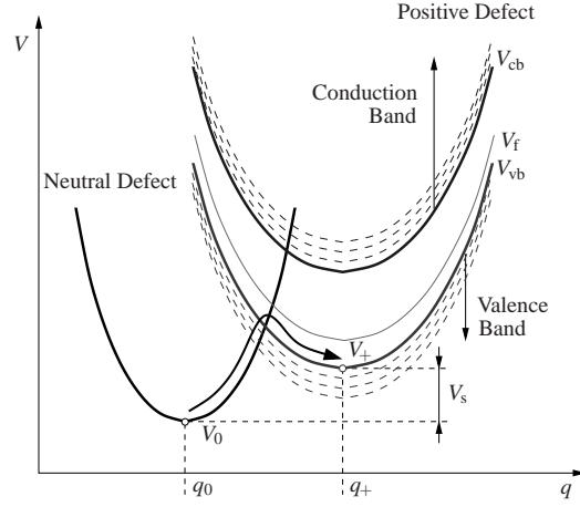
Fig. 5 A combined configuration coordinate diagram for hole capture and electron emission. According to the relation V_+ = \tilde{V}_0 + E , an electron located in an energetically higher band state E is represented by higher adiabatic potential V_+(q) . As a consequence, the upper and the lower family of curves constitute the set of adiabatic potentials V_+ associated with the conduction and valence band, respectively. It is noted that this configuration coordinate diagram remains unchanged for hole emission and electron capture and can therefore be used for both processes. As such, this diagram covers all possible NMP transitions of the considered defect with the substrate.
