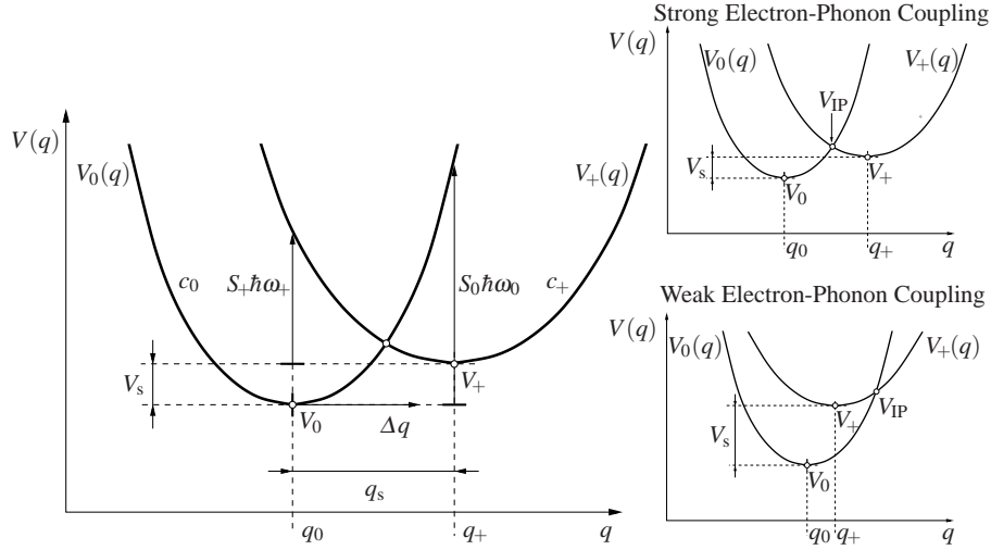
Fig. 8 Left: The configuration coordinate diagram including the Huang Rhys factors S_0 and S_+ . The adiabatic potentials are often defined as harmonic oscillators of the form V_0(q) = 1/2 M \omega_0^2 (q - q_0)^2 + V_0 and V_+(q) = 1/2 M \omega_+^2 (q - q_+)^2 + V_+ , where \omega_0 and \omega_+ are their respective oscillator frequencies. For an optical transition, the energy delivered by the photon must equal the energy difference V_0(q_+) - V_+ , which is indicated by the upwards arrow and can be expressed as an integral multiple S_0 of \hbar \omega_0 . In analogy, S_+ \hbar \omega_+ equals the energy difference V_+(q_0) - V_0 . In the remainder of this chapter, S_0 \hbar \omega_0 and S_+ \hbar \omega_+ will be replaced by S \hbar \omega and R^2 S \hbar \omega , respectively. Right: Strong (top) and weak (bottom) electron-phonon coupling. In the first case the parabolas are positioned such that the intersection point is situated inbetween their minima while in the second case one parabola lies inside the other and the intersection point is located beside the two minima.
