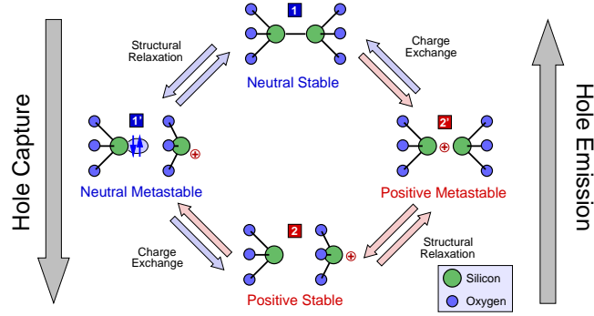
Fig. 10 (PRINT IN COLOR) State diagram of the multi-state model. The defect is present in a stable neutral (1) and a stable positive (2) charge state, where each of them has a second metastable state marked by a prime (1', 2'). The NMP transitions 1 \leftrightarrow 2' and 2 \leftrightarrow 1' occur between different charge states while the thermal transitions 1 \leftrightarrow 1' and 2 \leftrightarrow 2' between same charge states. Note that the transitions between the stable states are of main interest since they correspond to the experimentally measured capture and emission times in BTI. However, they involve intermediate states, which are metastable and important for the gate-bias and temperature dependence of the overall transition. The stick-and-ball models correspond to the configurations of a possible defect candidate, i.e. the oxygen vacancy, which is only shown for illustration purpose.
