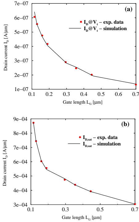
Fig. 1: Calibration of the threshold voltage V_t (a) and the saturation current I_{D,sat} (b) for NMOS devices created with 0.13 \mu\text{m} technology
