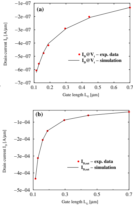
Fig. 2: Calibration of the threshold voltage V_t (a) and the saturation current I_{D,sat} (b) for PMOS devices created with 0.13 \mu\text{m} technology
