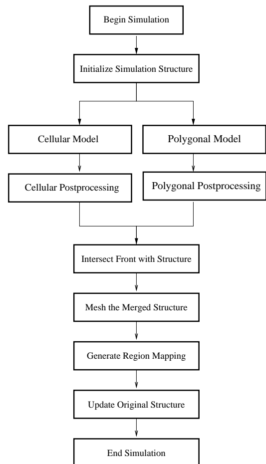
Fig. 1. Simulation flow of TOPO3D
