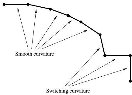
Fig. 4. Illustration of the point selection method in the smoothing stage
