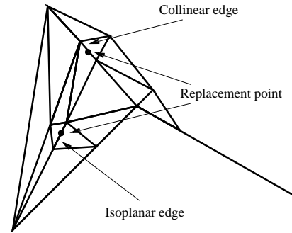
Fig. 6. Illustration of the edge removal algorithm in the coarsening stage
