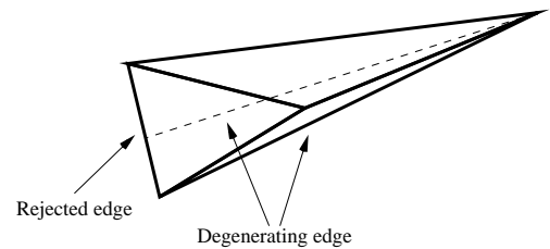
Fig. 7. Example for an edge which degenerates the surface triangulation if it would be removed
