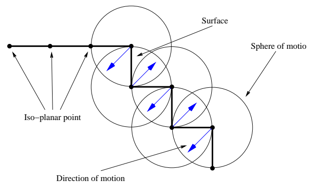
Fig. 3. Illustration of the point offset mechanism in the smoothing stage
