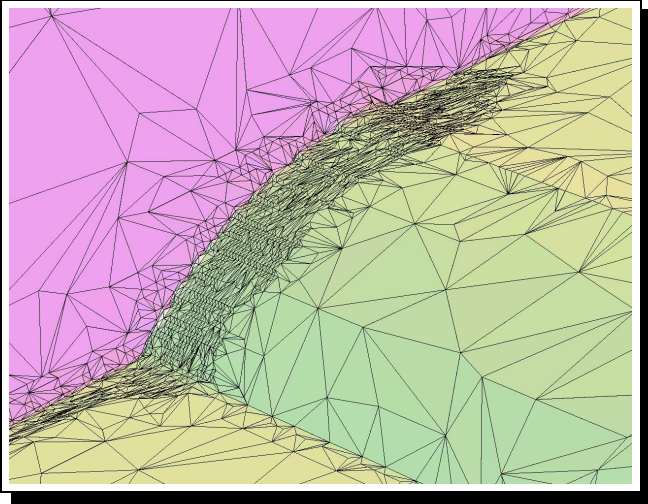
Fig. 8. Process front after applying the coarsening stage (24302 triangles)
