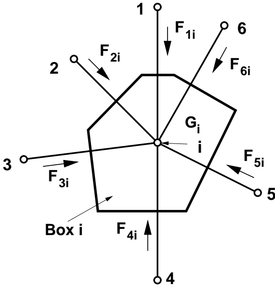
Figure 2: Box i with 6 neighbors
