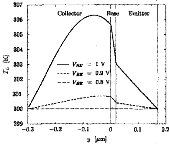
Fig. 3. Lattice temperature distribution of an HBT with the isotherm contact model for different bias voltages.
