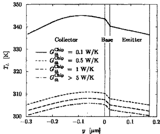
Fig. 4. Lattice temperature distribution of an HBT for different thermal contact conductances.
