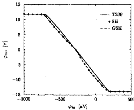
Fig. 12. Comparison of the open-loop gain of the \mu\text{A} 709 for the T300, SH and GSH model.
