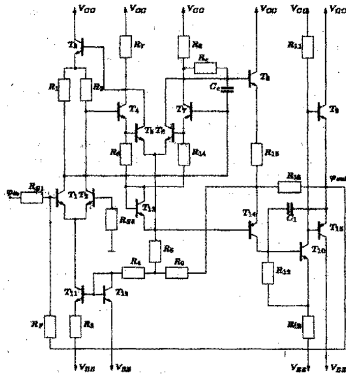
Fig. 10. Schematic of the \mu A 709 OpAmp.
