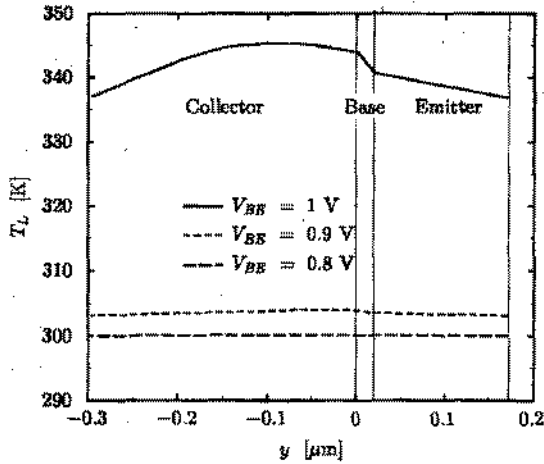
Fig. 6. Lattice temperature distribution of an HBT with the contact resistance model for different bias voltage.
