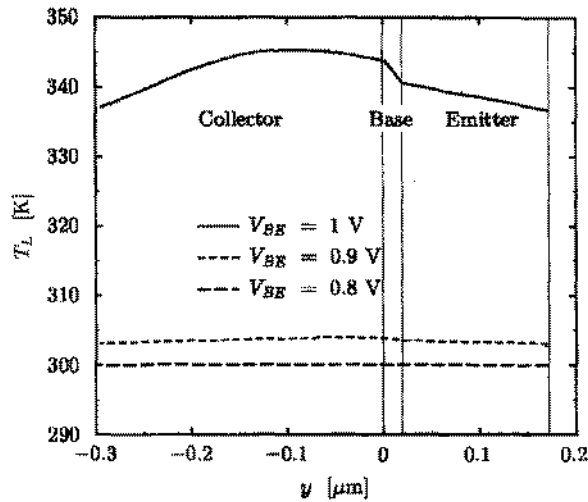
Fig. 5. Heat generation distribution of an HBT for different thermal contact conductances.
