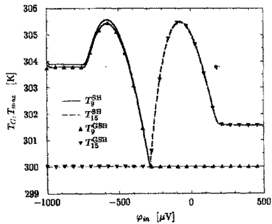
Fig. 14. Maximum and contact temperature of the output transistors T_9 and T_{15} during the DC transfer characteristic for both self-heating model.
