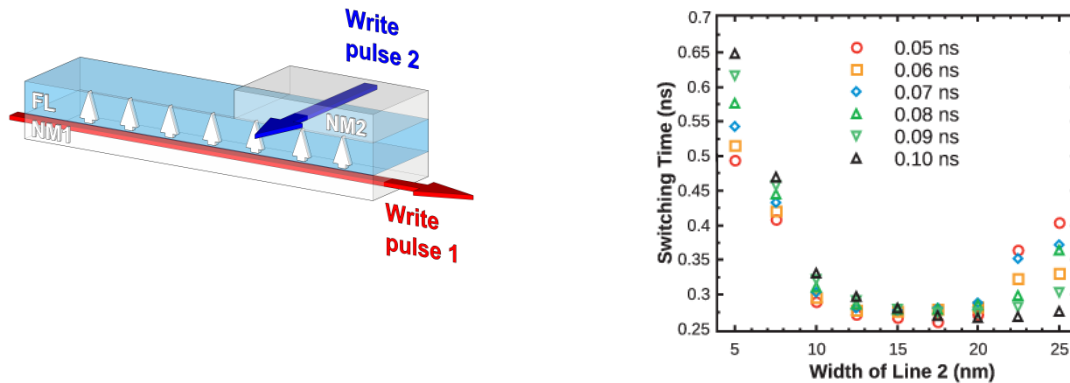
FIG. 1. (a) Perpendicular SOT-MRAM memory cell with a 52.5x12.5x2 nm free layer; (b) Switching time vs. line 2 width, for several durations of the pulse 2, I_1 = I_2 = 100 \mu\text{A} .
